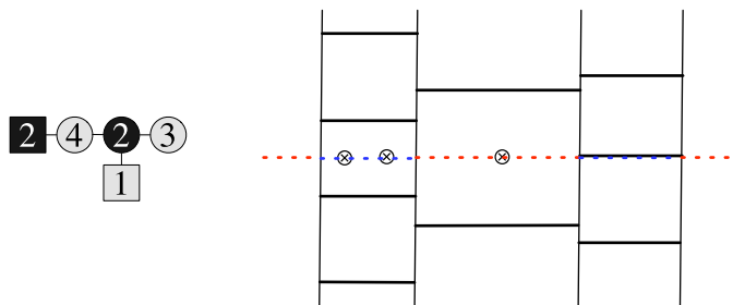
Figure 3. On the left: an example of SO–USp quiver gauge theory. A circle or a box stands for a gauge group or a flavor symmetry, respectively. A gray object with n inside is an SO(n) group, a black object with n inside is a USp(n) group. On the right: the brane configuration realizing the quiver. The vertical lines stand for NS5-branes, the horizontal lines D4-branes suspended between them, and \otimes D6 branes. The dotted line represents the O4-plane. The color distinguishes two types of O4-planes.
