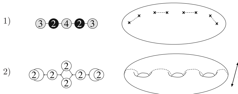
Figure 9. An \text{SO}(4)\text{--USp}(2) quiver and the same quiver as an \text{SU}(2) generalized quiver. Corresponding G -curves are also shown. In the first description the curve is a sphere with eight punctures; in the second it is a hyperelliptic genus-three curve.
