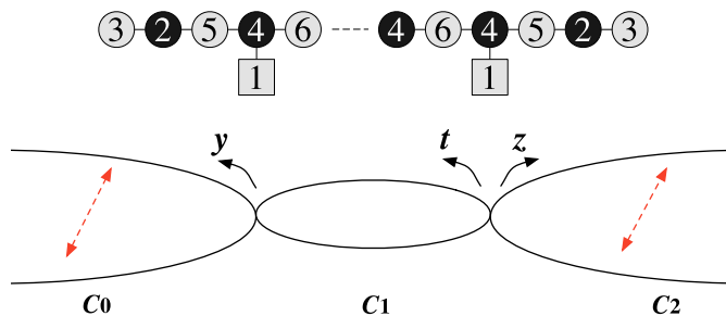
Figure 11. A quiver, and the corresponding Taub-NUT space in which its Seiberg-Witten curve is embedded. Orientifolding fixes C_1 , but acts as multiplication by -1 on C_0 and C_2 .
