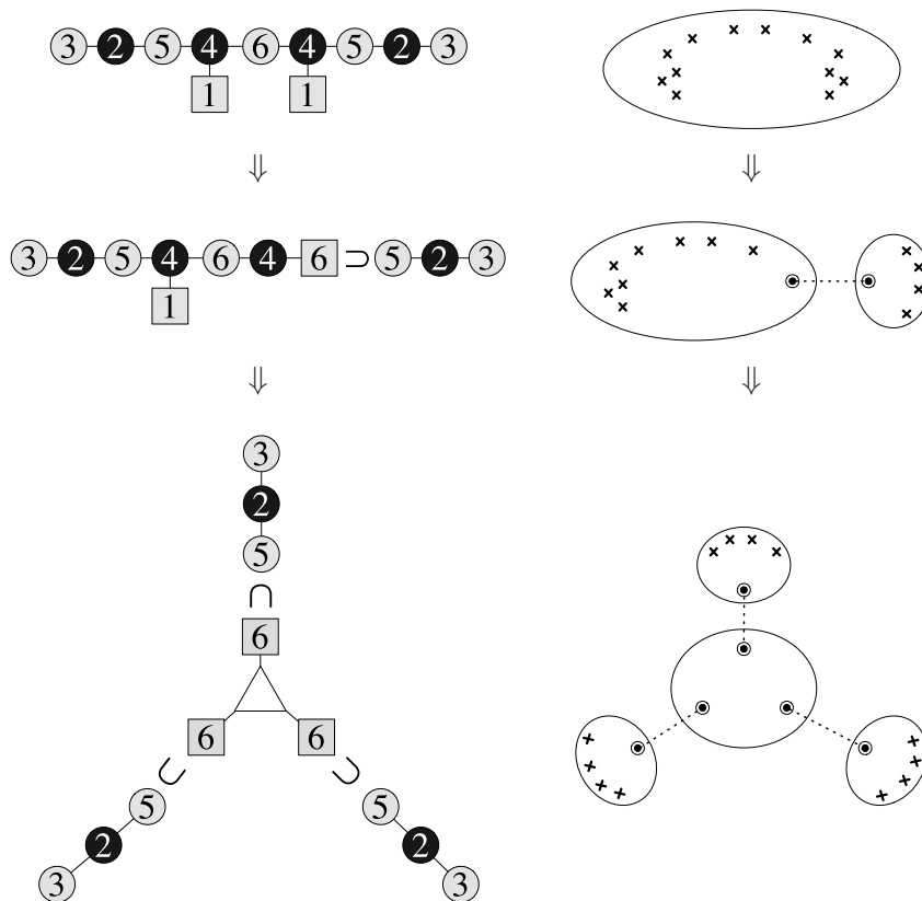
Figure 5. Construction of T_{SO(6)} . The triangle with three SO(6) flavor symmetries attached stands for the T_{SO(6)} . The symbol \subset between the SO(6) flavor symmetry and the SO(5) gauge symmetry signifies that SO(5) \subset SO(6) is gauged.
