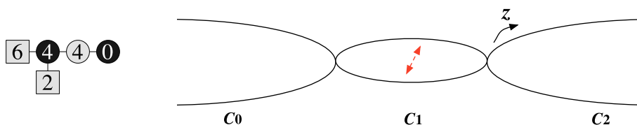
Figure 12. Another quiver, and the corresponding Taub-NUT in which its Seiberg-Witten curve is embedded. Orientifolding fixes C_0 and C_2 , but acts as multiplication by -1 on C_1 .
